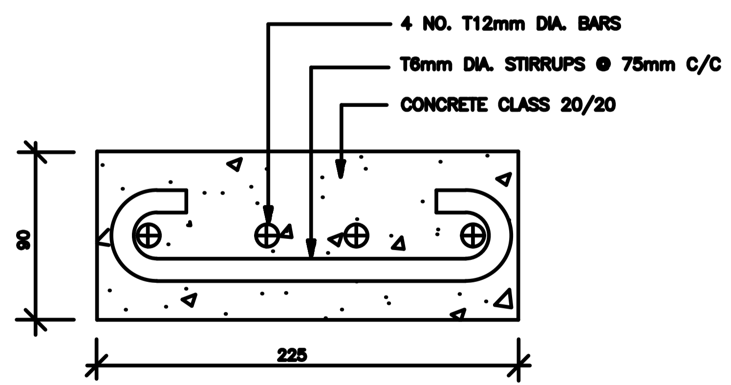
SECTION Y-Y SCALE 1:5
