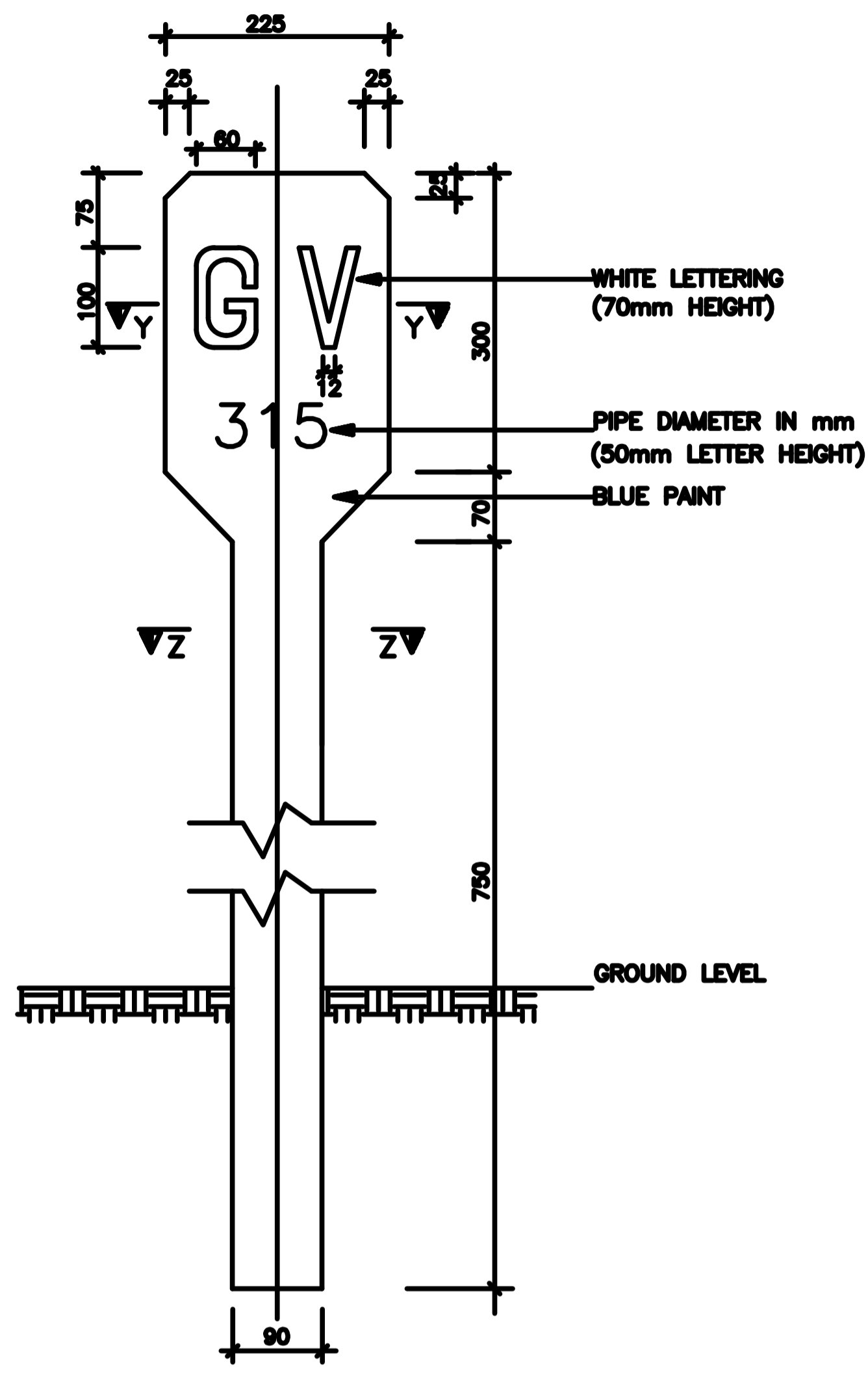
GATE VALVE INDICATOR POST SCALE 1:5
