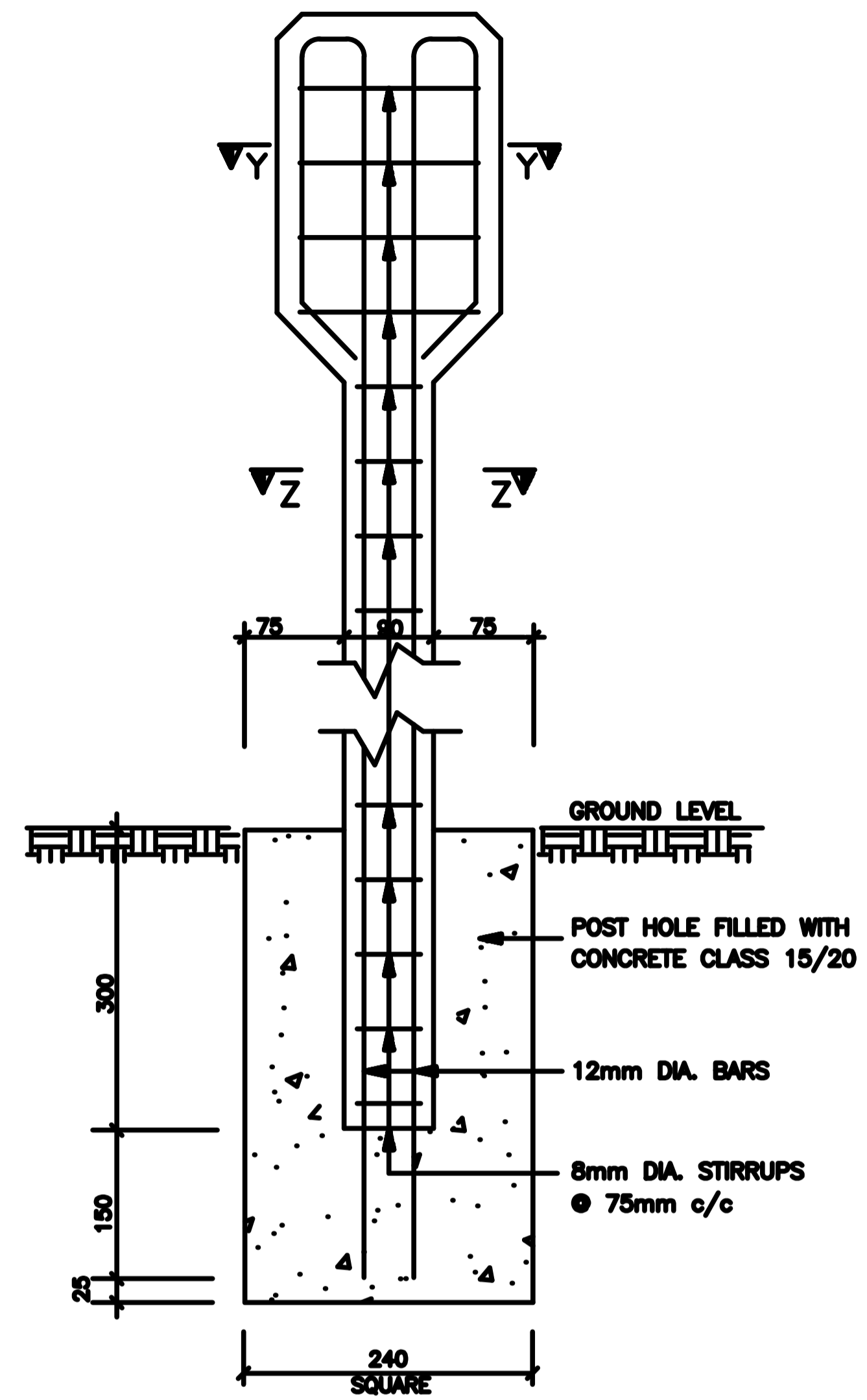
INDICATOR POST REINFORCEMENT DETAILS SCALE 1:5
