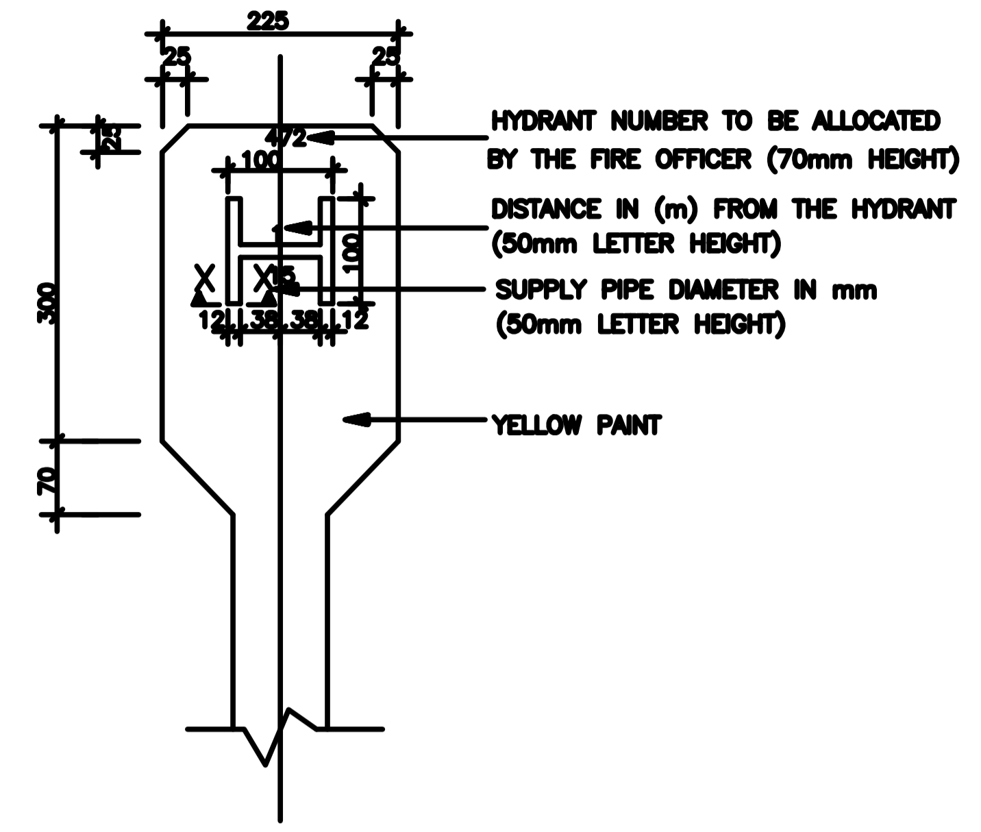
FIRE HYDRANT POST SCALE 1:5
