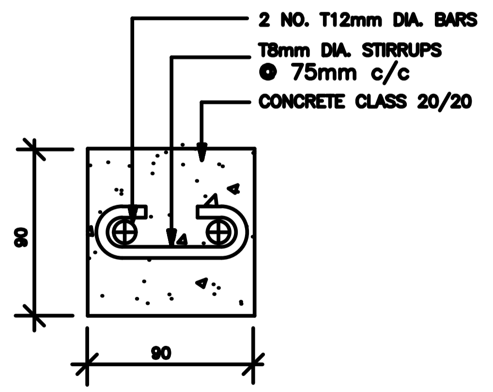
SECTION Z-Z SCALE 1:5
